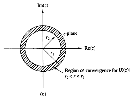
Figure 3.1 Region of convergence for X(z) and its corresponding causal and anticausal components.
